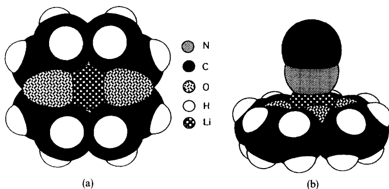
Fig. 6. Optimised structures of (a) the (12-crown-4)· \text{Li}^+ complex with D_{2d} symmetry and (b) the (12-crown-4)· \text{Li}(\text{NCS}) complex with C_{4v} symmetry.
